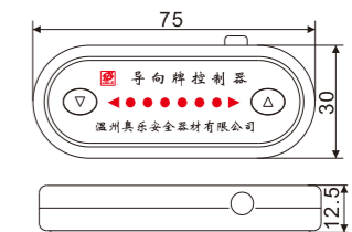
JDX-K2 Arrow board Controller
