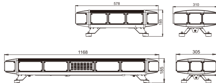
TBD-50L12A-48
